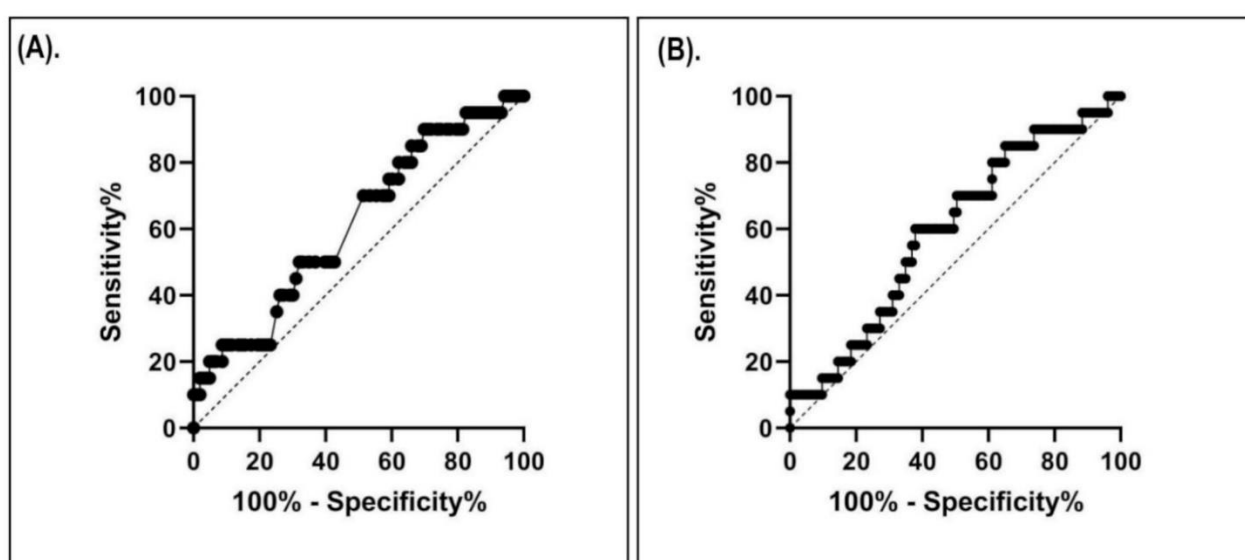
Figure 2. The ROC between albumin levels and platelet – to albumin ratio and the risk of peritonitis among patients with peritoneal dialysis. A). Albumin levels. B). Platelet – to albumin ratio.
